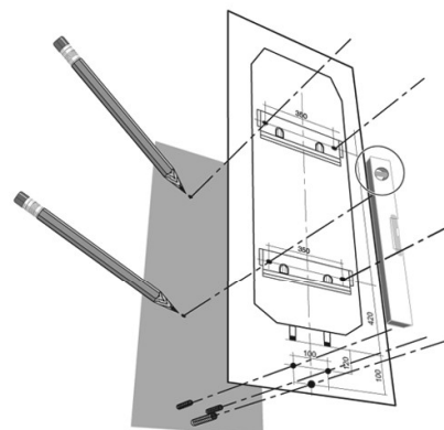
TR5500T 120... | 150...
